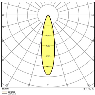
FL PFM 200W 4000K SYM R30 BK
